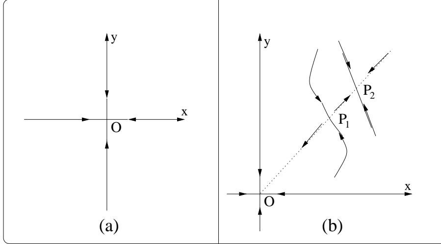
FIGURE 7. The Phase Portraits for the FitzHugh-Nagumo Equation: a) the local map has two fixed points ( O is attracting, \infty is repelling); b) the local map has four fixed points ( O and P_2 are attracting, P_1 is saddle, and \infty is repelling).
