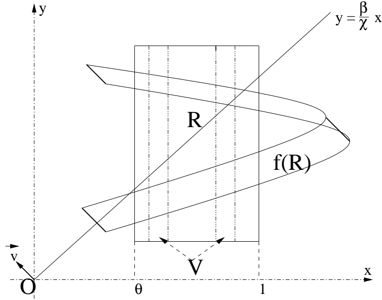
FIGURE 3. The Horseshoe for the Local Map of the FitzHugh-Nagumo Equation
