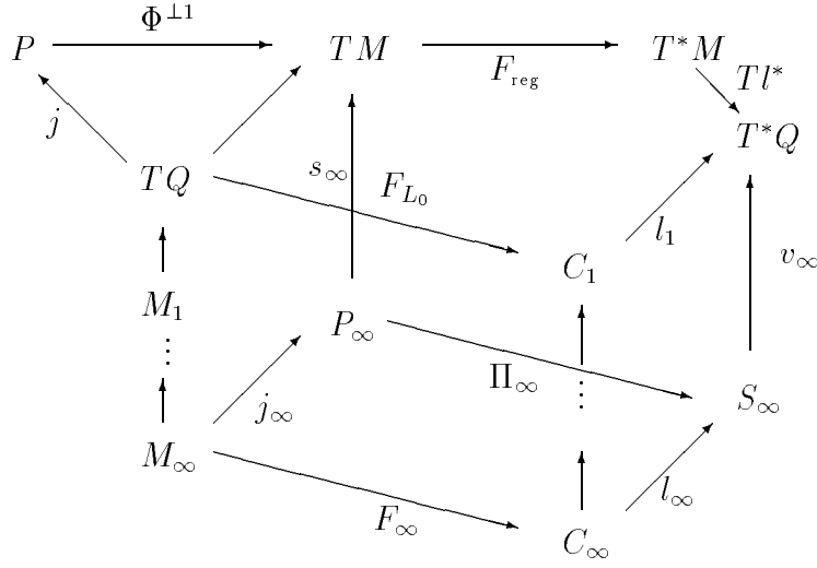
Figure 2: Lagrangian regularization and Dirac's theory of constraints.
